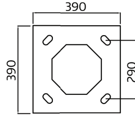
BASE PLATE
