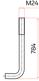
M24 x 864 Anchor Bolts ... 4 pcs
